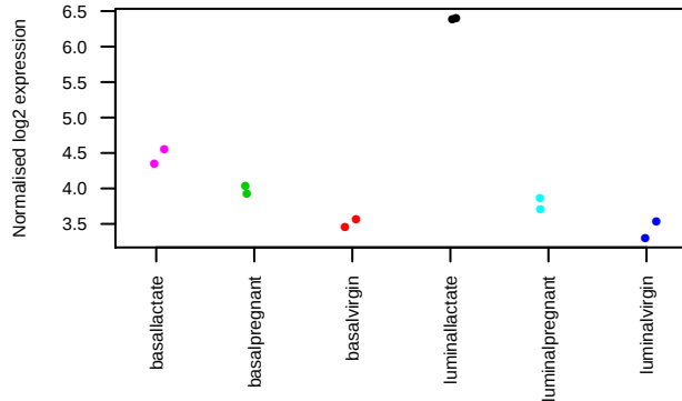
Slc33a1 logFC=-2.6, adj.P.Val=0.00052
