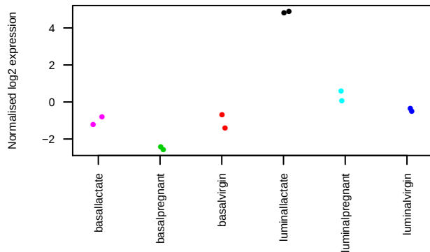
Ttyh1 logFC=-4.55, adj.P.Val=0.00052
