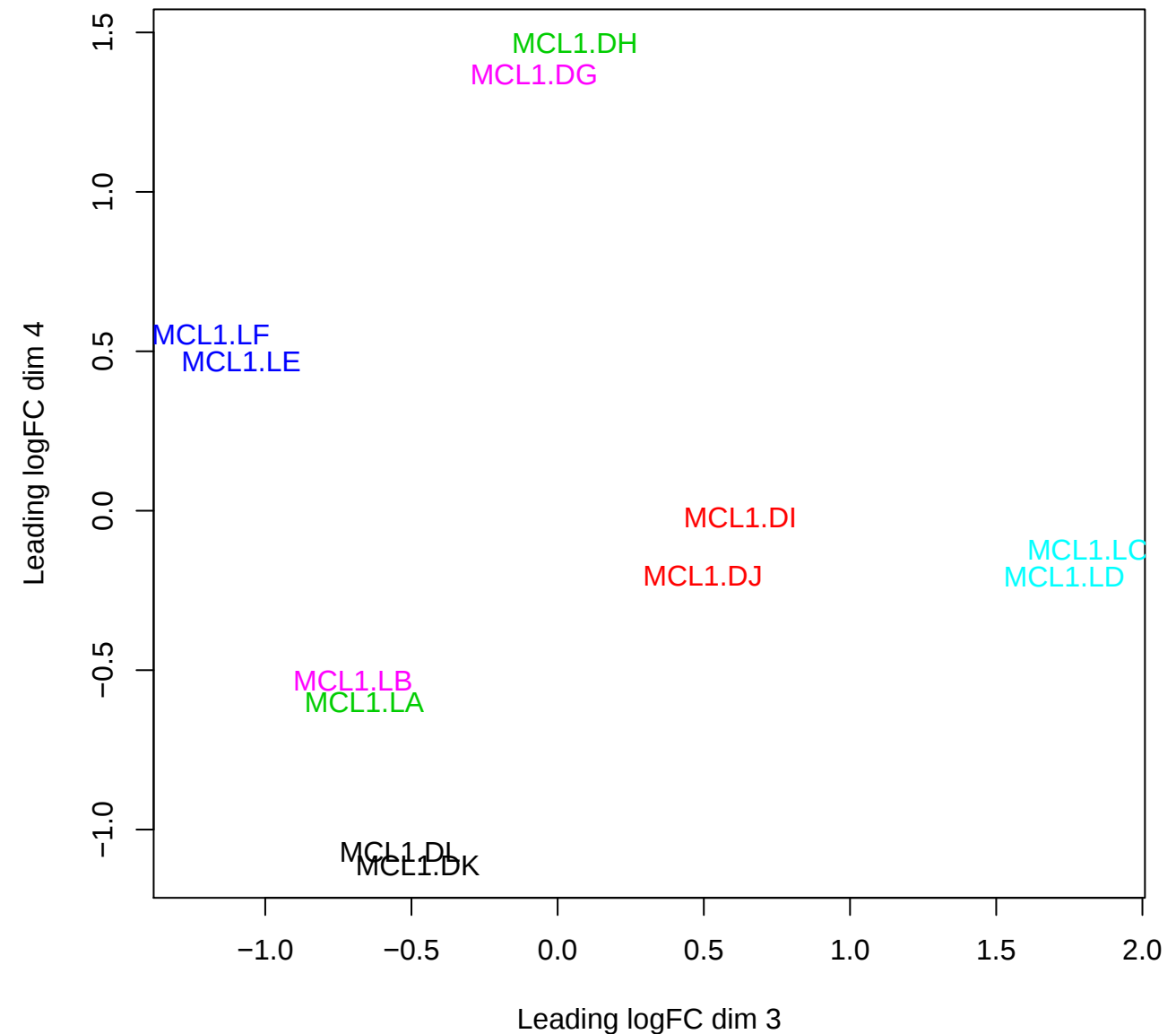
MDS Plot: Dims 3 and 4
