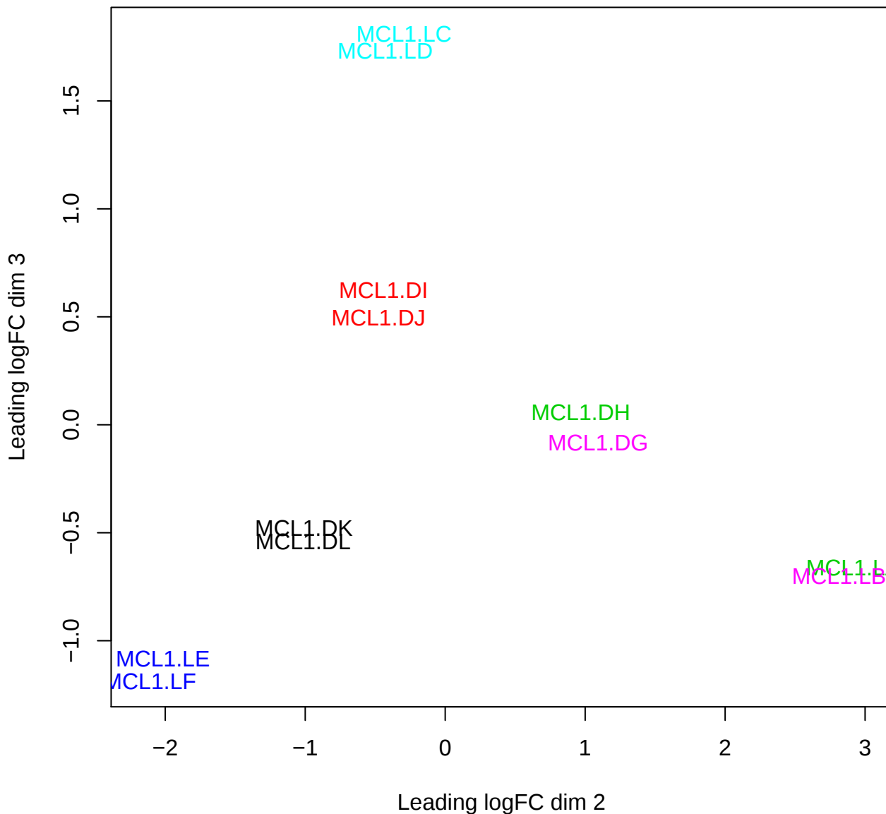
MDS Plot: Dims 2 and 3
