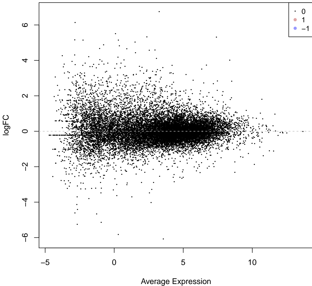
MD Plot: basalpregnant-basallactate
