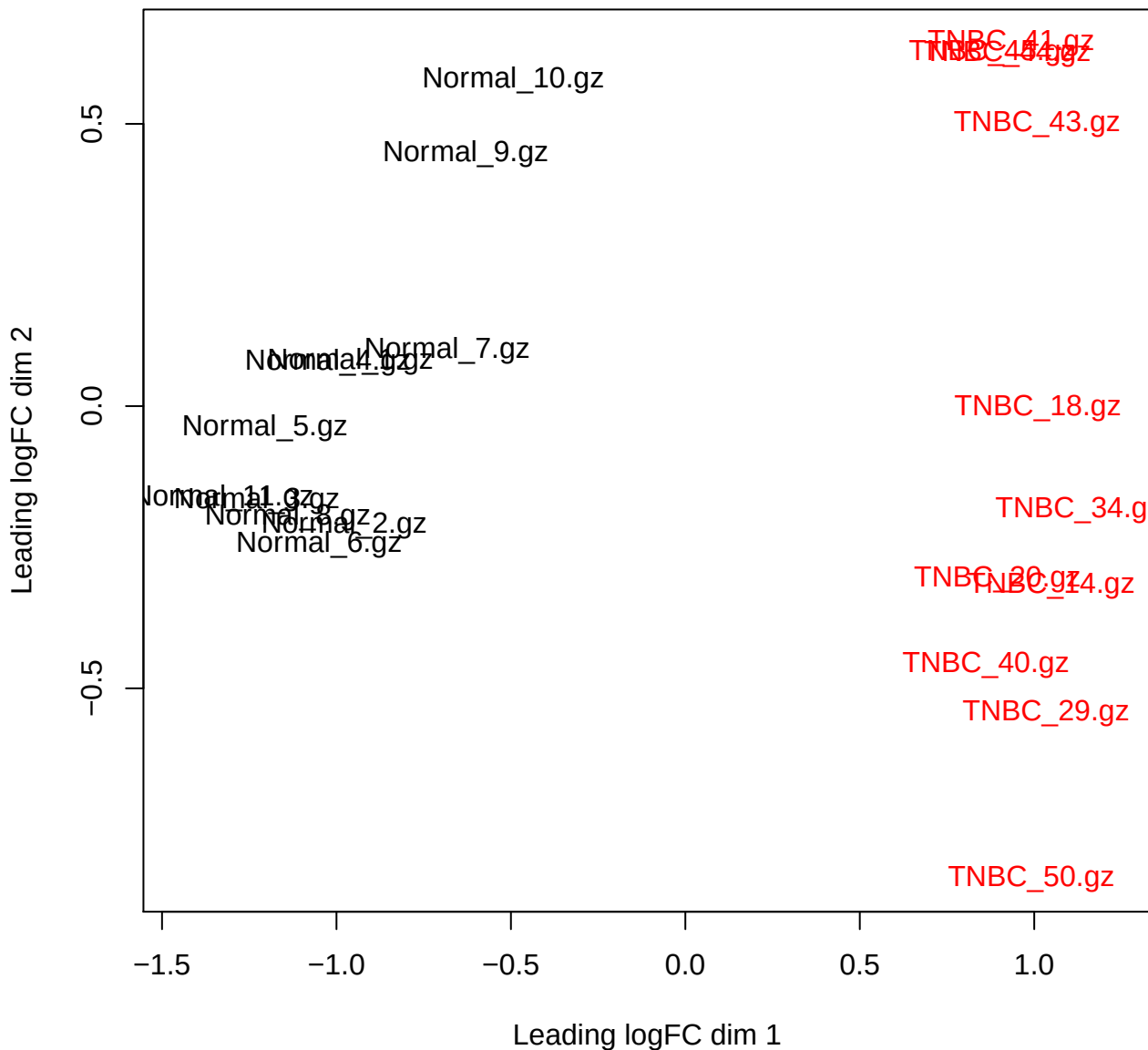
MDS Plot: Dims 1 and 2
