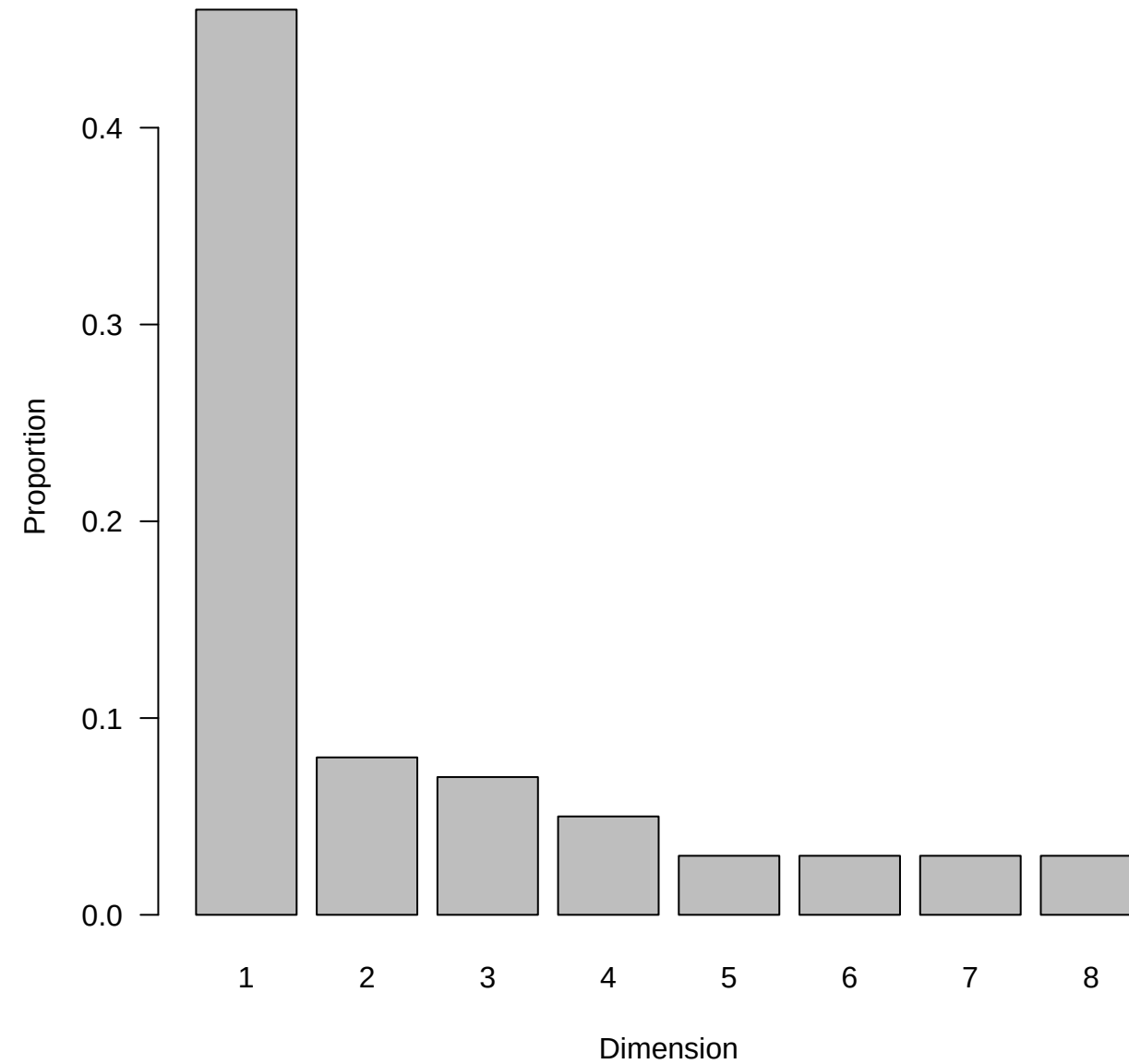
Scree Plot: Variance Explained
