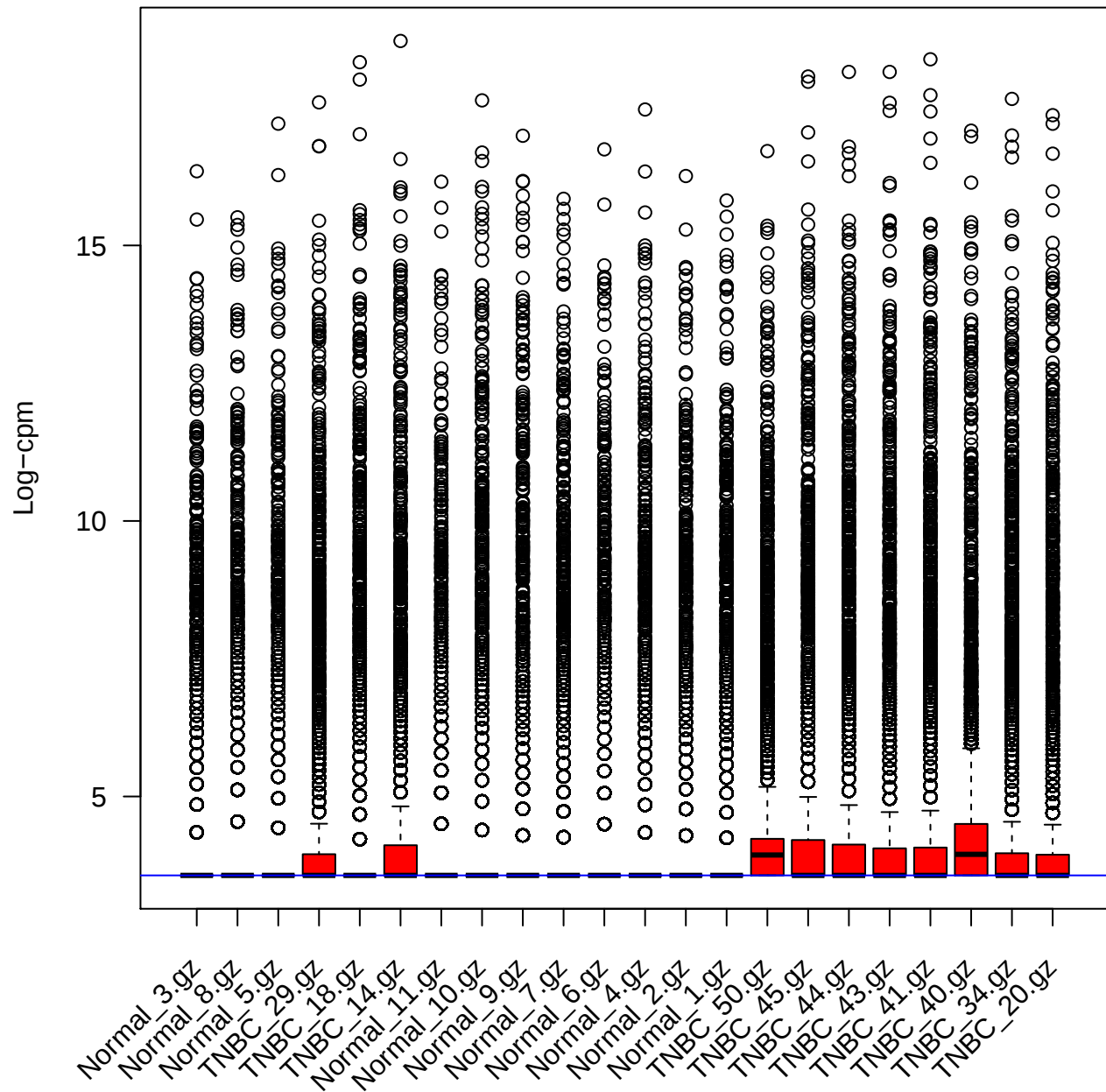
Box Plot: Normalised counts
