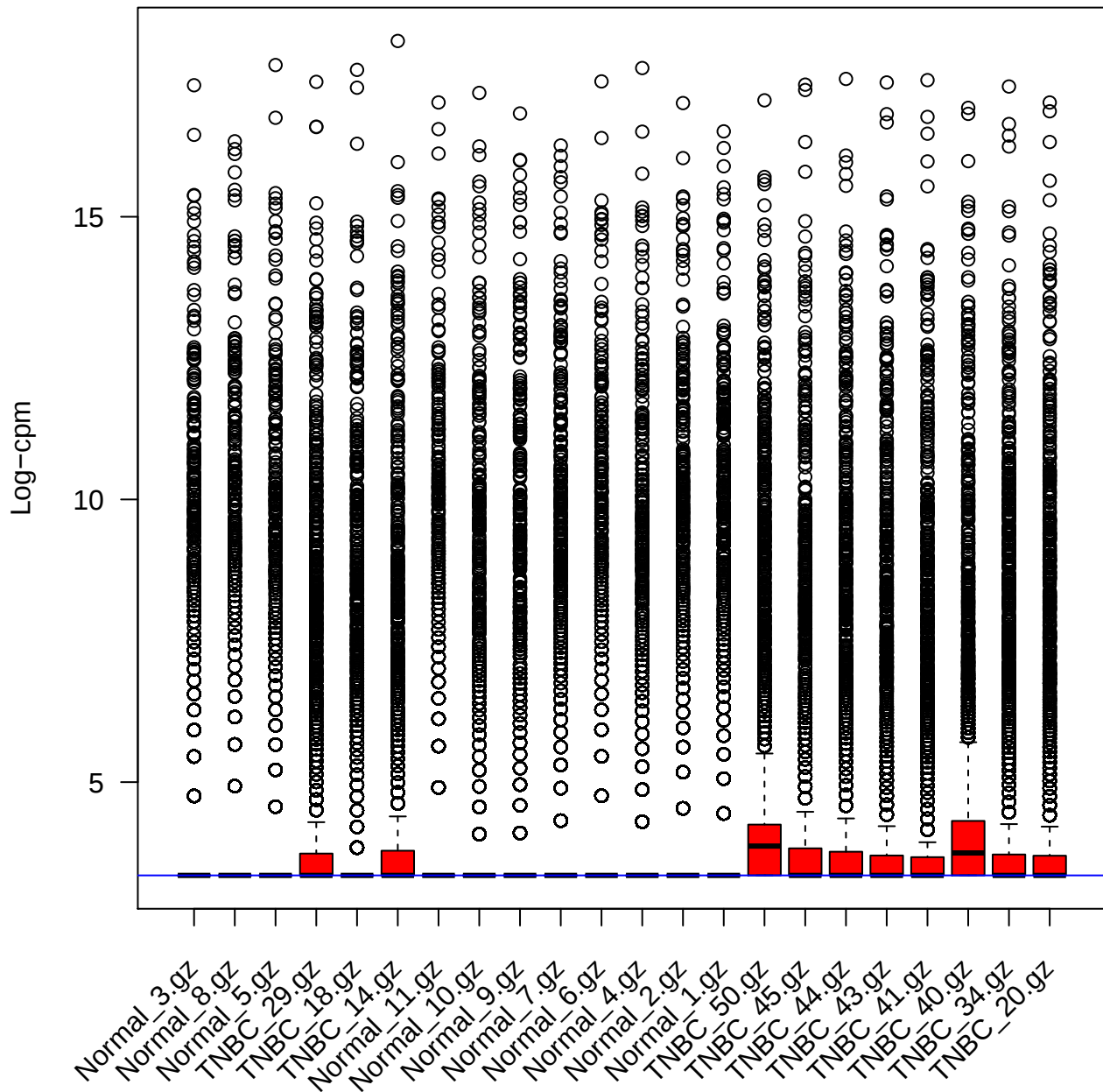
Box Plot: Unnormalised counts
