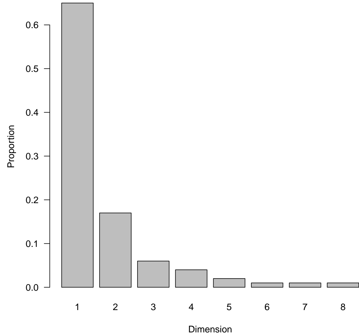
Scree Plot: Variance Explained
